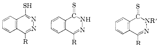
IXa, R = H b, R = C 6 H 5 c, R = CH 3 XIa, R = H; R' = C 6 H 5 b, R = R' = C 6 H 5 c, R = CH 3 ; R' = C 6 H 5
